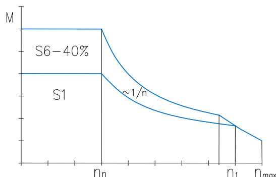
TORQUE DIAGRAM
