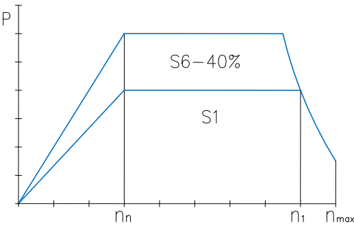
POWER DIAGRAM
