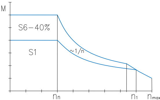
TORQUE DIAGRAM
