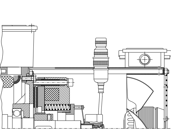
BRAKE ASSEMBLY
