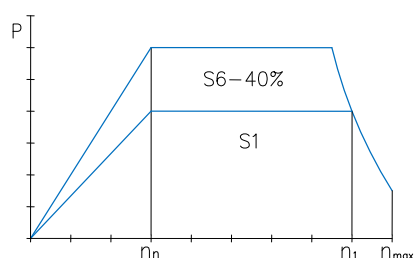
POWER DIAGRAM
