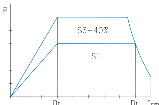
POWER DIAGRAM
