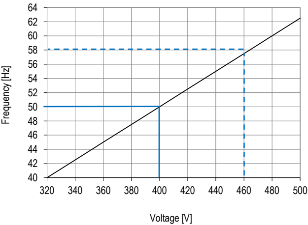
VOLTAGE/FREQUENCY DIAGRAM
