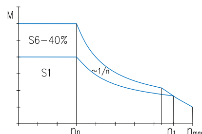
TORQUE DIAGRAM
