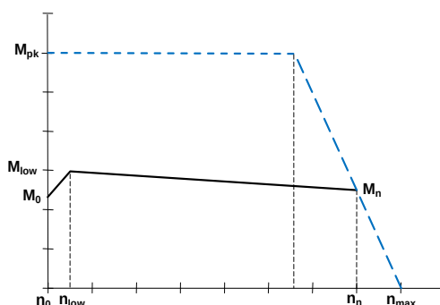
TORQUE DIAGRAM
