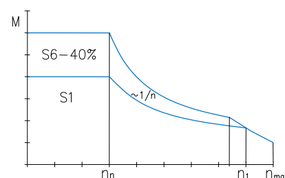
TORQUE DIAGRAM
