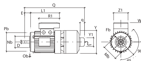
BAE 160/180/200/225 B3
