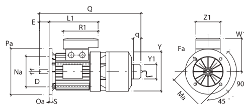
BAE B14
